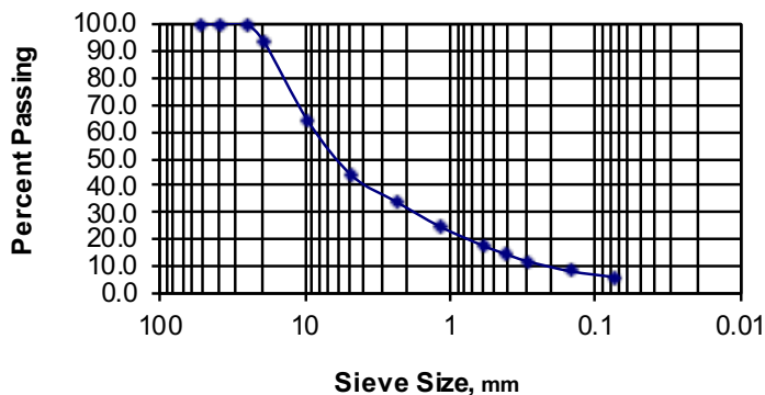
Grainsize Distribution Curve
